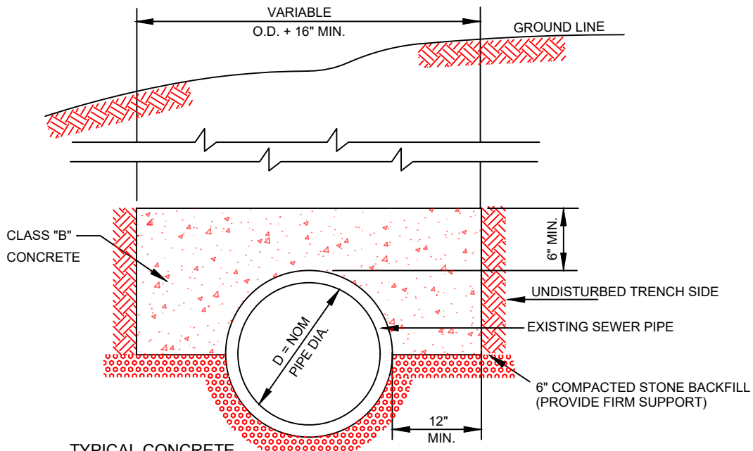
TYPICAL CONCRETE PROTECTION FOR NEW SEWERS
