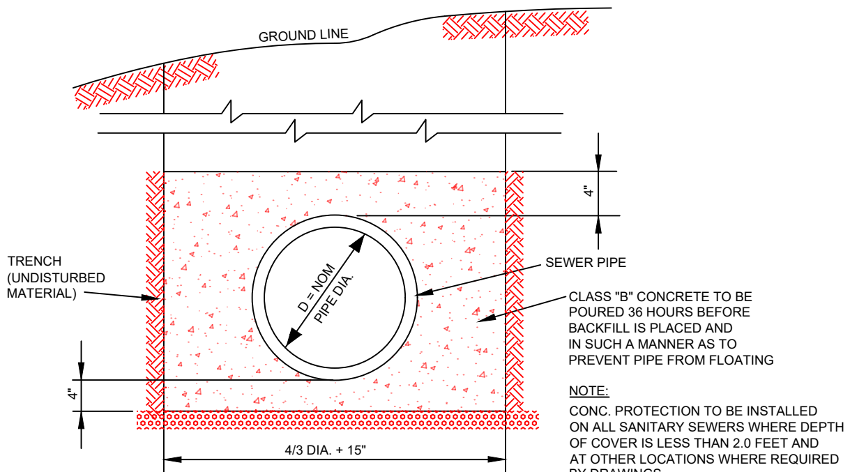
TYPICAL CONCRETE PROTECTION FOR NEW SEWERS
