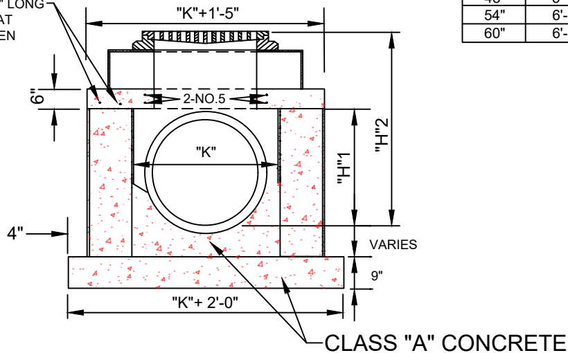
SECTION "A"
