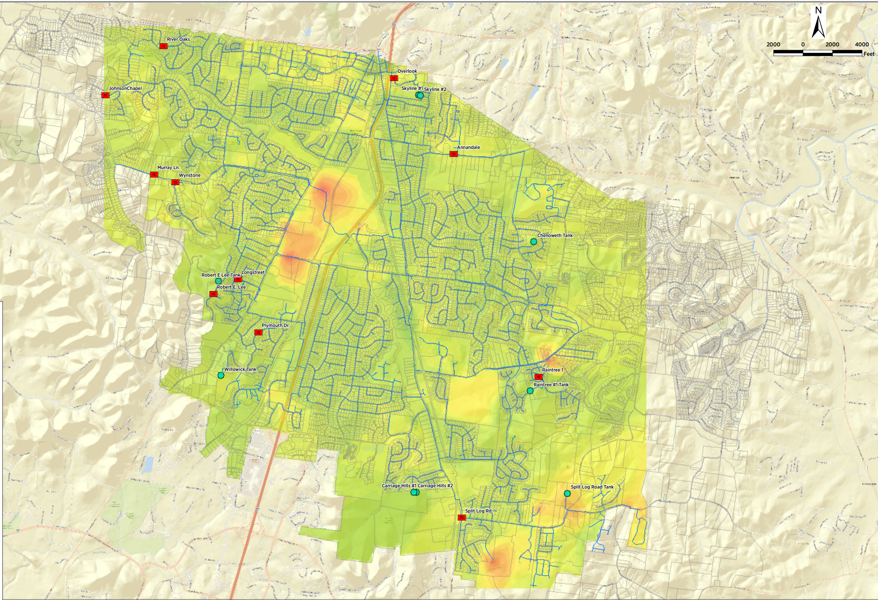
Long Term Max. Demand
