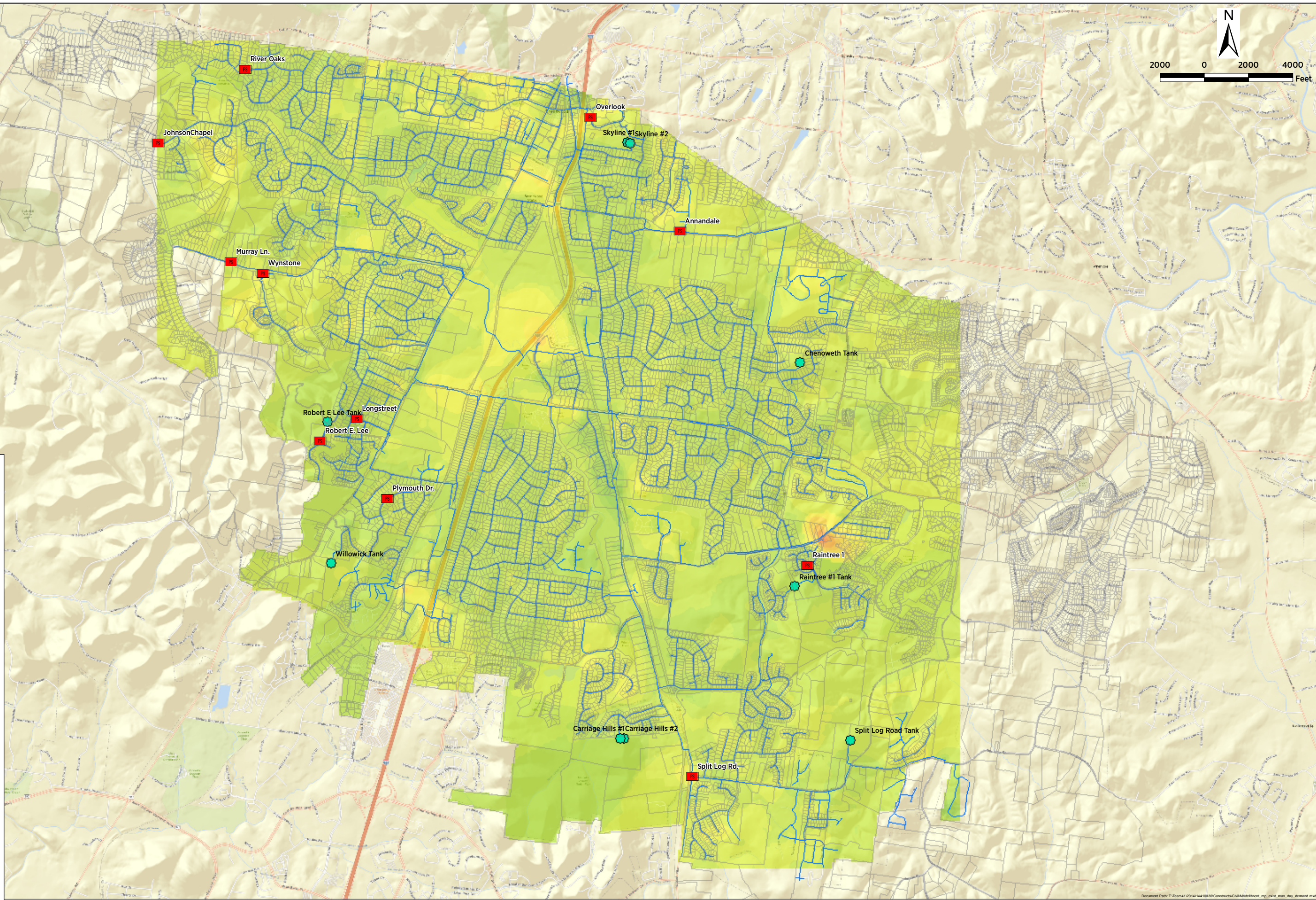
Existing Max. Demand
